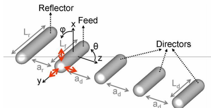
Fig. 1. Overview of the nano-optical Yagi-Uda antenna. For an operating wavelength of 570 nm and an aluminum antenna ( \epsilon = -38.0 + i10.9 ), the feed element is resonant for L_f = 160 nm. The director length ( L_d ) is 0.9L_f , the reflector length ( L_r ) is 1.25L_f . The director spacing ( a_d ) is \lambda/4 , the reflector spacing ( a_r ) is \lambda/4.4 . Red arrows represent x-, y- and z-oriented dipolar emitters and are placed at the location of efficient coupling to the feed element.
