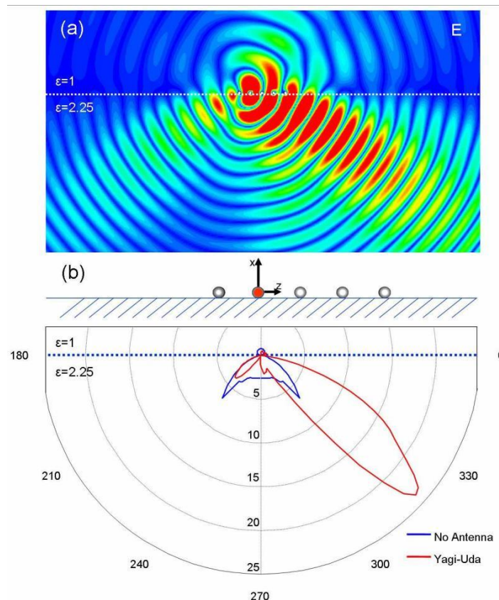
Fig. 5. A y-oriented emitter coupled to a lossless Yagi-Uda antenna (distance 4 nm, L_f = 187 nm) placed on a dielectric substrate ( \epsilon = 2.25 ). (a) Snapshot of the local field (xz plane). Movie of full cycle is available as supporting information. (b) The angular directivity. The substrate fills the half-space from \theta = 180^\circ to 360^\circ . The situation without antenna is shown as a reference. The emission is directed in a single lobe into the substrate.
