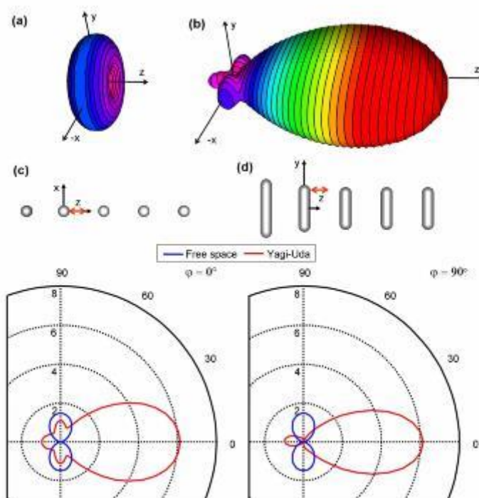
Fig. 3. Directivity for a z-oriented emitter in (a) free space and (b) coupled to a Yagi-Uda antenna (distance 3 nm). (c), (d) directivity in the major planes. The schematics show the position of the emitter and the orientation of the emitter and antenna relative to the image plane. The emission of the coupled system is highly directed and rotated by 90 degrees.
