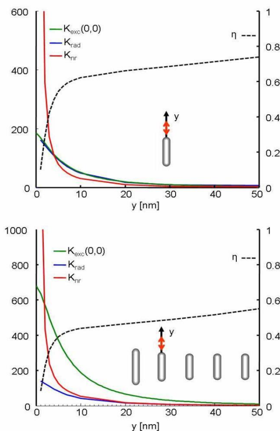
Fig. 4. The distance dependence of the excitation, K_{exc}(0,0) , radiative, K_{rad} , and non-radiative, K_{nr} , rates and the efficiency, \eta , for a y-oriented dipole coupled to a dipole and to a Yagi-Uda antenna. The insets show the position and orientation of the emitter relative to the dipole respectively Yagi-Uda antenna.
