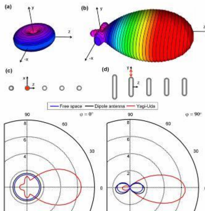
Fig. 2. Directivity for a y-oriented dipolar emitter in (a) free space and (b) coupled to a Yagi- Uda antenna. (c), (d) the directivity in the two major planes. As a reference the emitter coupled to a dipole antenna is added. The schematics show the location of the emitter and the orientation of the emitter and Yagi-Uda antenna relative to the image plane. The distance between the emitter and the antenna element is 4 nm. The emission of the emitter coupled to the Yagi-Uda antenna is highly directed.
